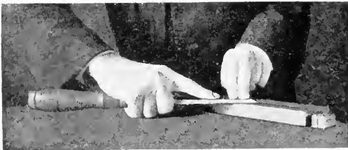
Fig. 23. Removing the Wire Edge from the Plain Side of a Chisel.
